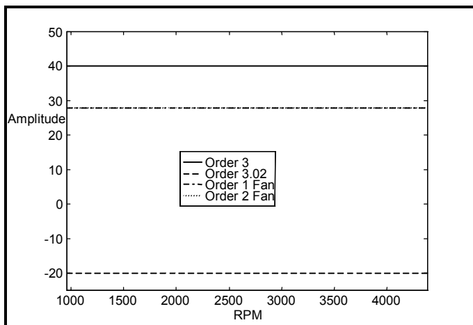
Figure 8: TVDFT constant order bandwidth estimates with OCM compensation.
