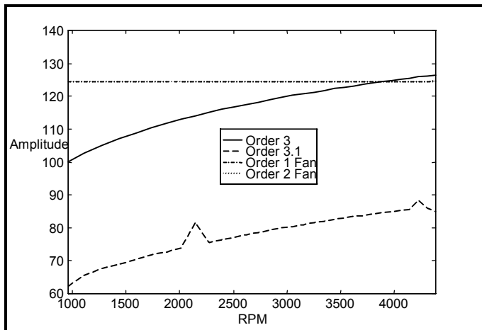
Figure 7: TVDFT constant order bandwidth estimates with OCM compensation.
